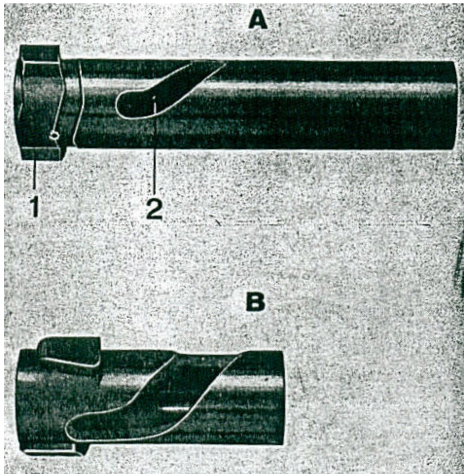
Figure 10 Locking Sleeve
