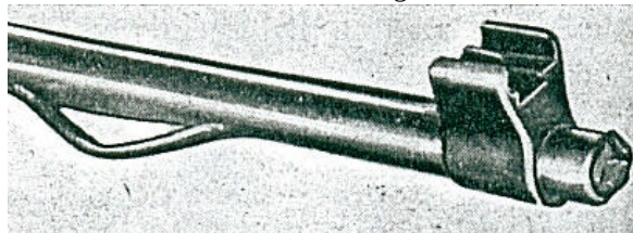
Blocked, exploded barrel
