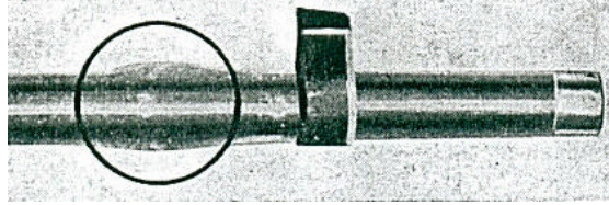
Bulged Barrel
