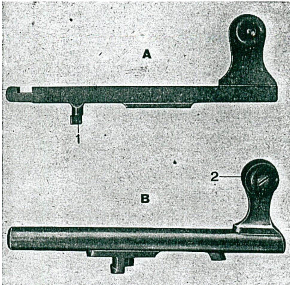
Figure 8 Cam Follower
