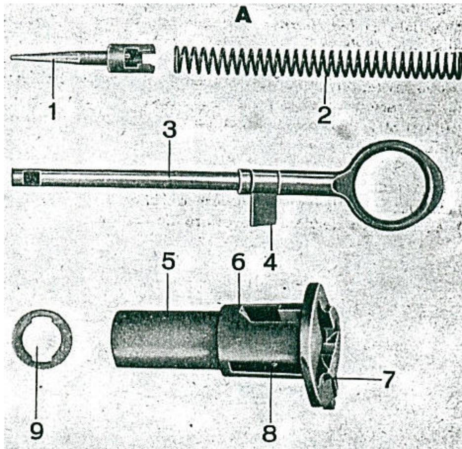
Fig. 11 Firing Mechanism
