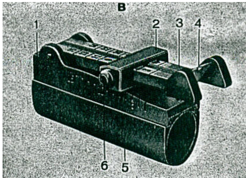
Figure 5 Rear Sight
