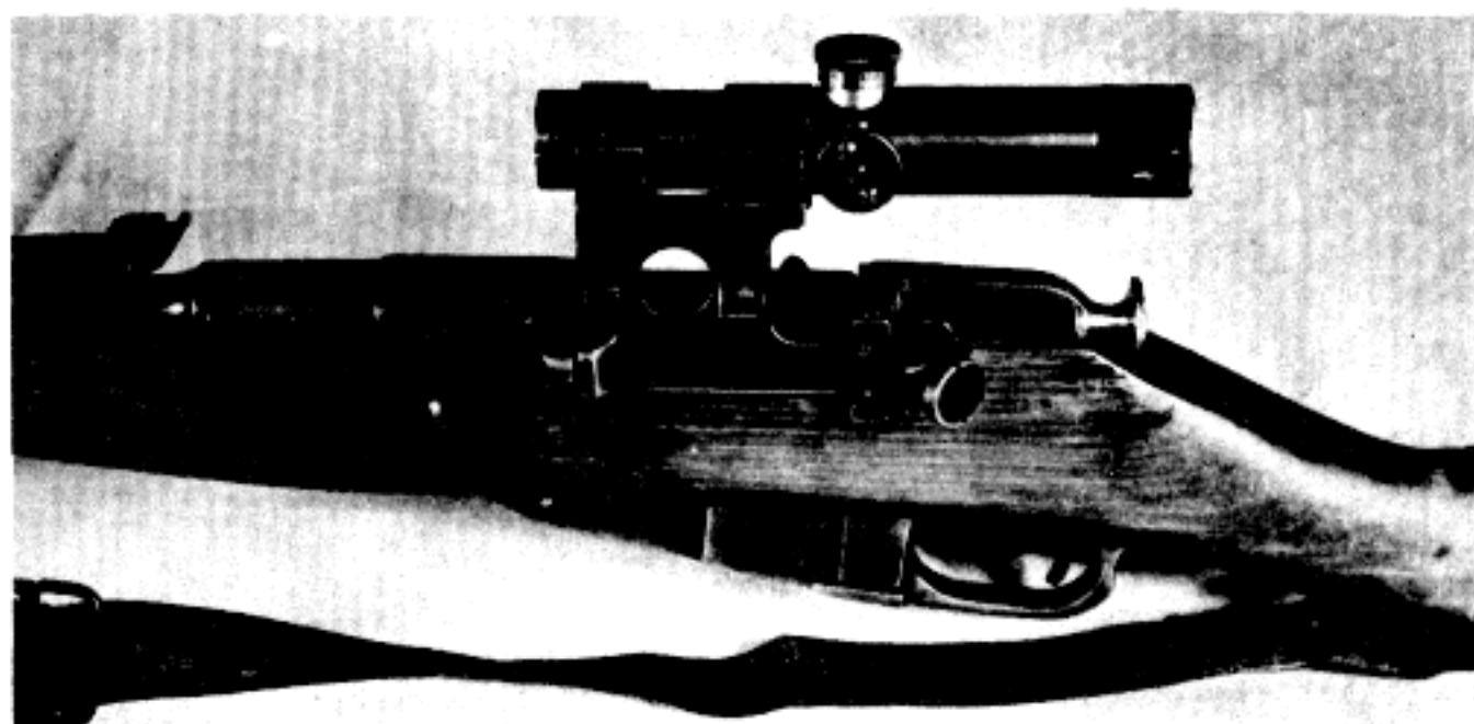
FIGURE 27. SNIPER RIFLE WITH PU TELESCOPE AND MOUNT (RIGHT SIDE).
