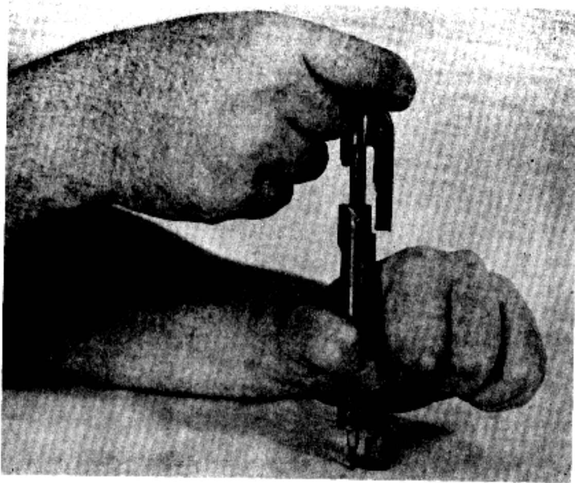
FIGURE 47. REMOVING COCKING PIECE.
