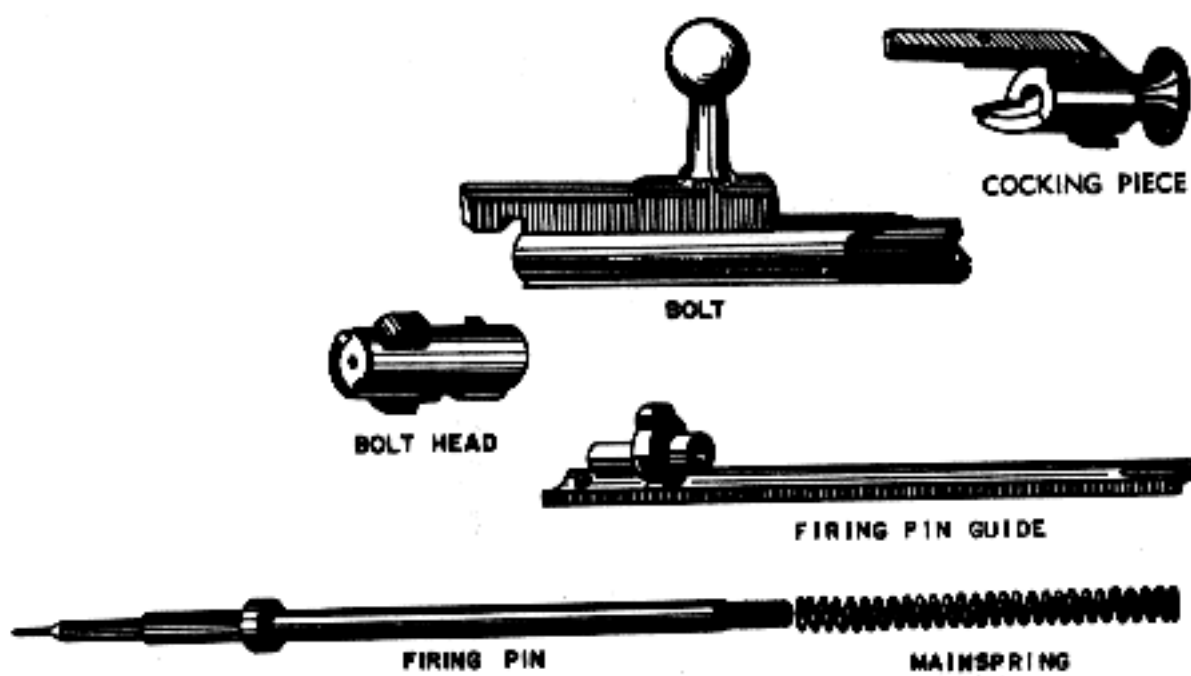
FIGURE 48. BOLT ASSEMBLY COMPONENTS.
