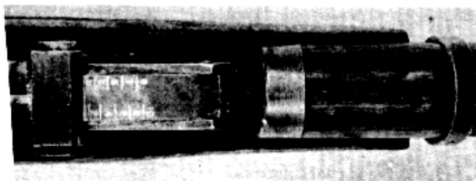
FIGURE 31. REAR RAMP SIGHT FOR CARBINE M1938.
