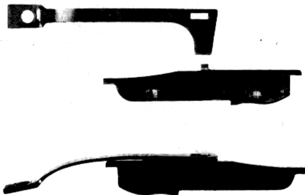
FIGURE 21. TWO-PIECE INTERRUPTER-EJECTOR FOR RIFLE M1891/30.
