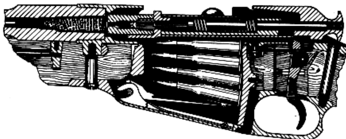
FIGURE 38. POSITION OF PARTS AFTER RIFLE IS LOADED.
