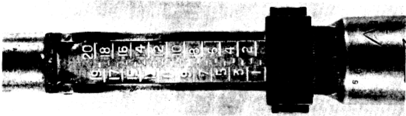
FIGURE 17. REAR SIGHT FOR RIFLE M1891/30 (TOP VIEW).
