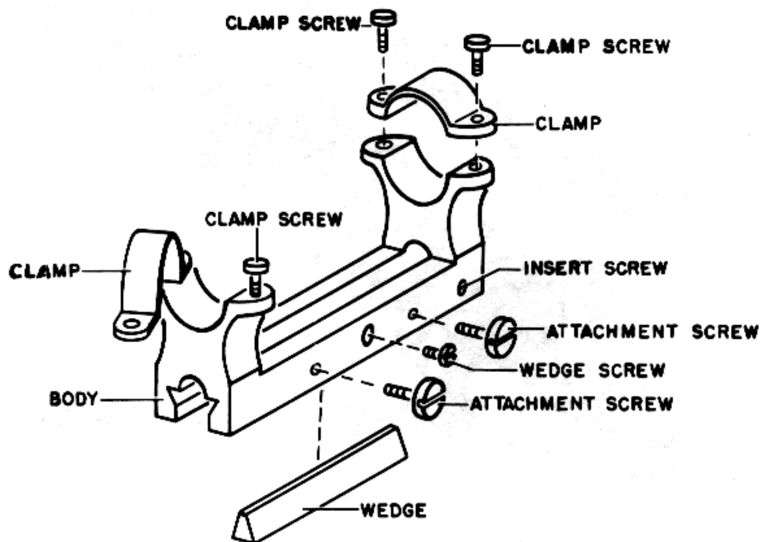
FIGURE 25. BODY OF PE TELESCOPE MOUNT.
