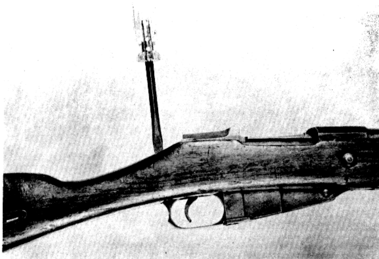
FIGURE 49. REMOVING REAR TRIGGER GUARD SCREW.
