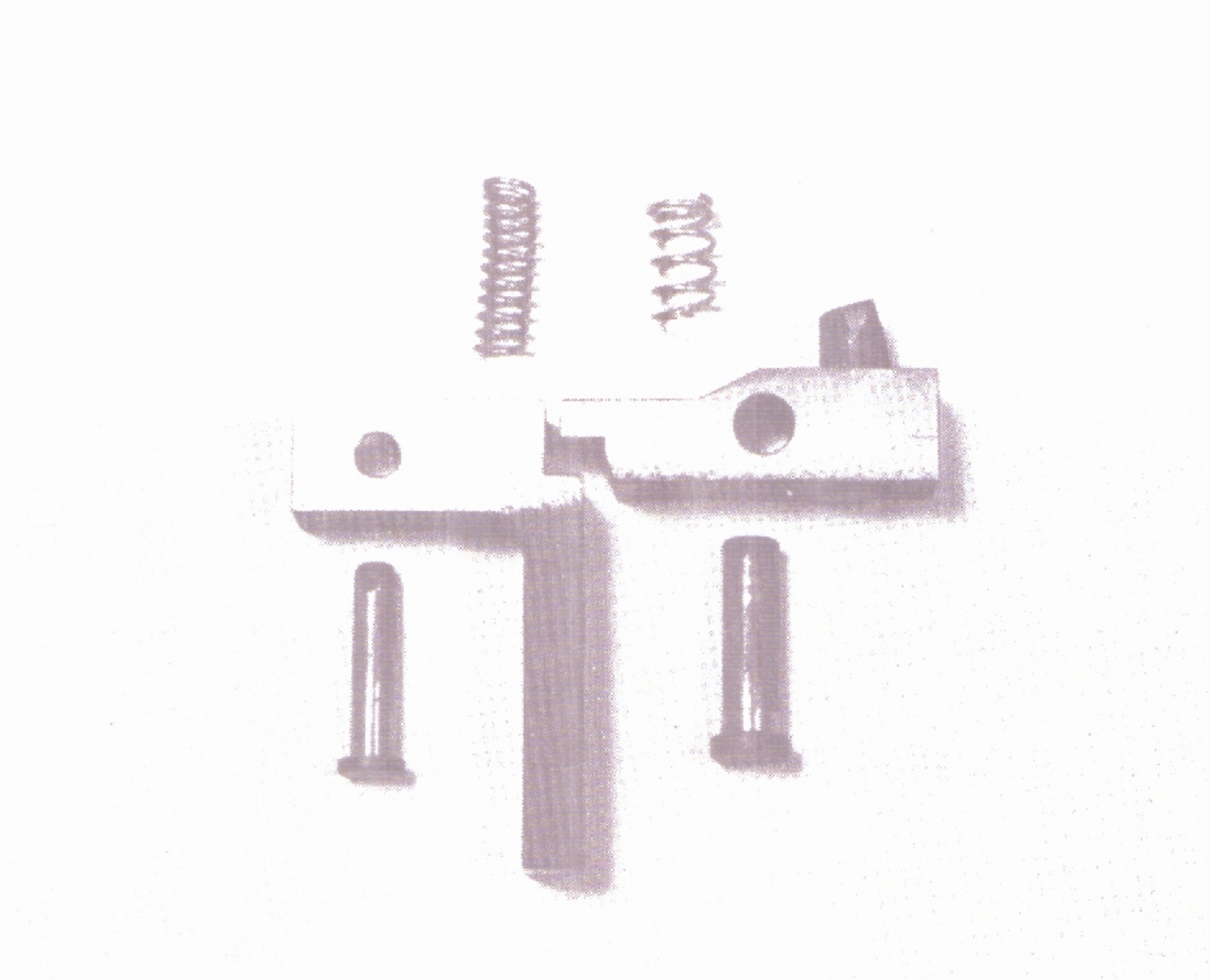
The complete trigger/sear mechanism. Being devoid of a safety and select fire option, the mechanism is the ultimate in simplicity.
