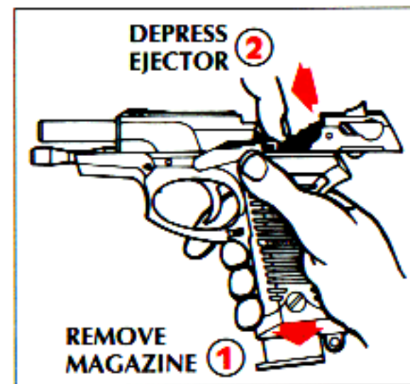
FIGURE 3 Press slide stop up. Depress ejector.
