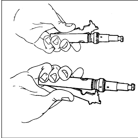
Figure 3-21. Cleaning of the gas regulator plug grooves.
