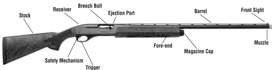
PICTURE 1 This picture shows the main parts of a REMINGTON AUTOLOADING SHOTGUN.
