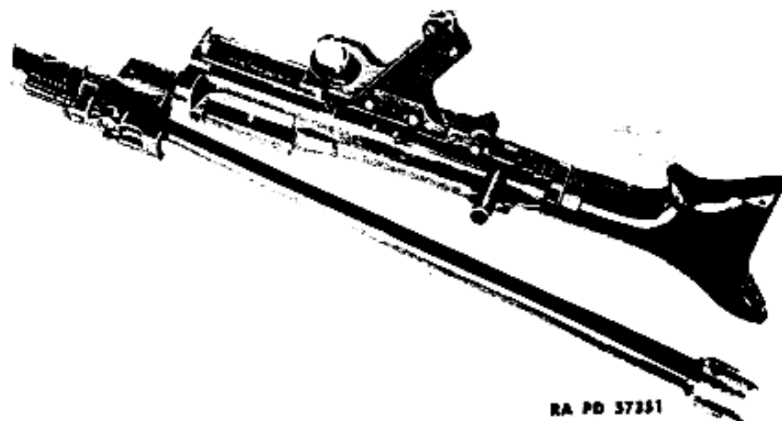
Figure 40 — Sliding Barrel out of Barrel Casing
