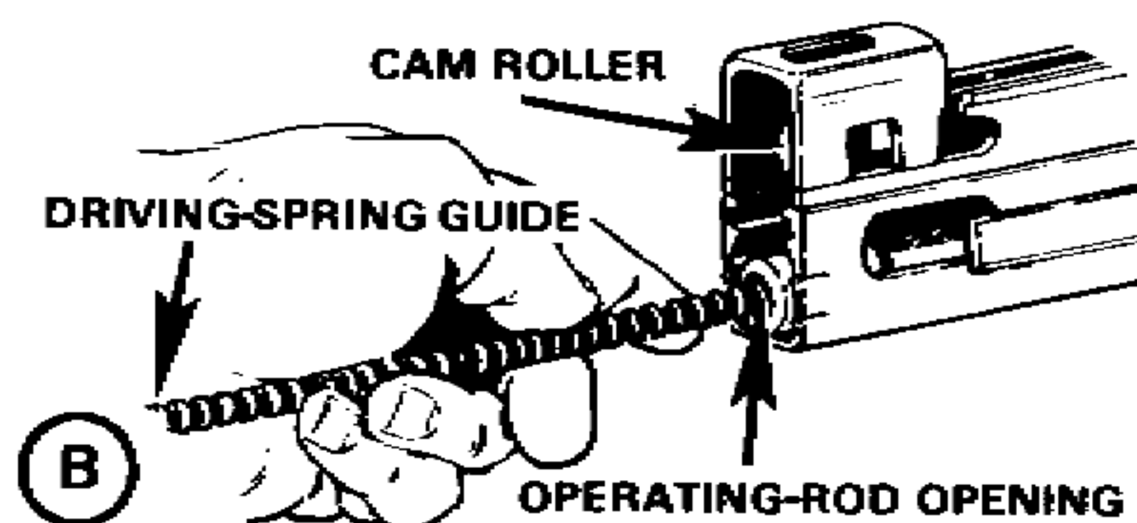
INSERTING THE DRIVING SPRING
