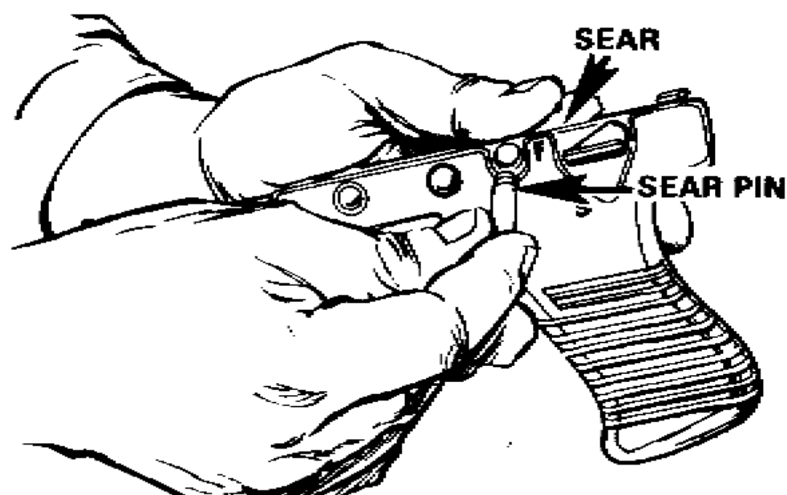
(C) REMOVING THE SEAR RETAINING PIN
