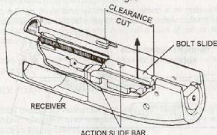
Fig. 10 — Bolt slide removal
