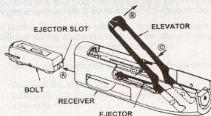
Fig. 11 — Elevator removal
