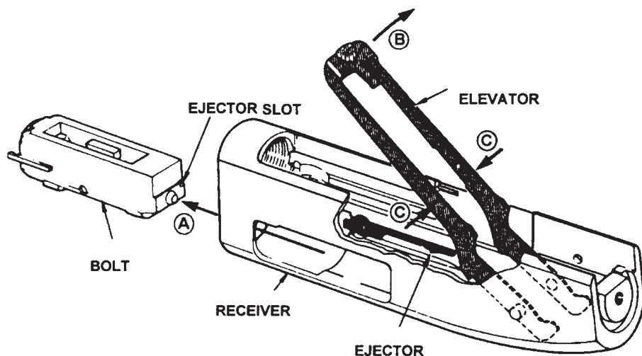
Fig. 11 – Elevator removal
