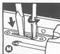
Turning rivet to lock ejector down
