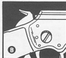
Half Cock
