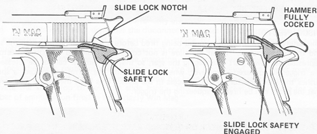
Illust. No. 2— SLIDE LOCK SAFETY
