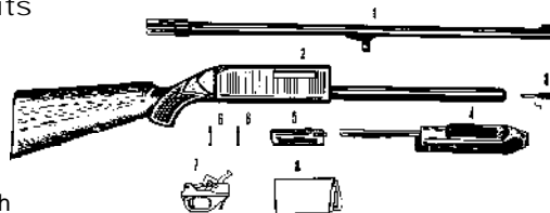
Fig. 5 - IZH81M or KM Version with Folding Stock
