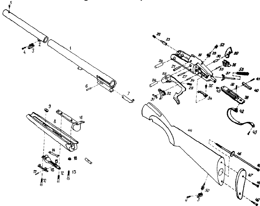
Fig. 1 - IZH18 Exploded View
