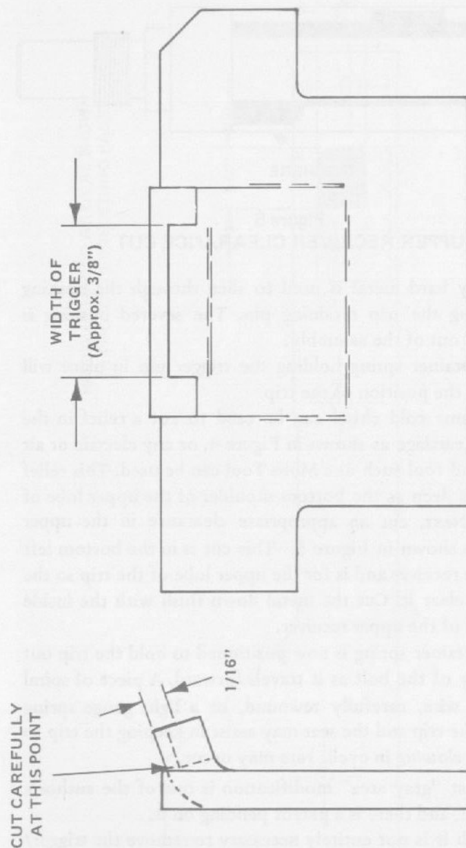
Figure 6 .45 ACP FEED RAMP CUT
