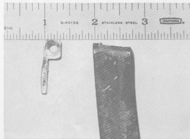
Finished auto sear with original rough stock.
