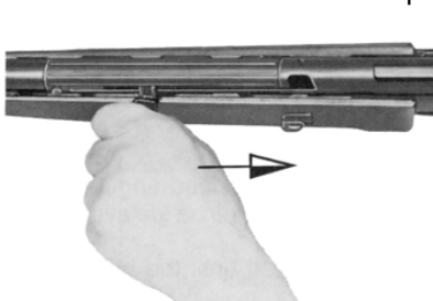
Fig. 32 Retracting the cocking lever
