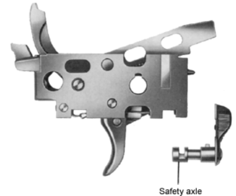
Fig. 16 Trigger mechanism and safety
