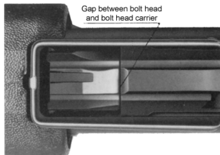
Fig. 41 Head space
