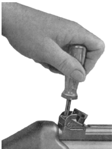
Fig. 43 Loosening of clamping screw
