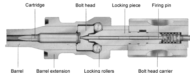
Fig. 34 Bolt in locked position
