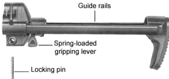
Fig. 18 Retractable buttstock
