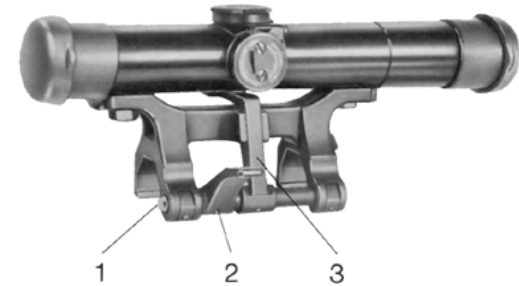
Fig. 53 Telescopic sight with mount
