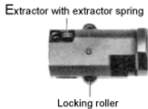
Fig. 11 Bolt head
