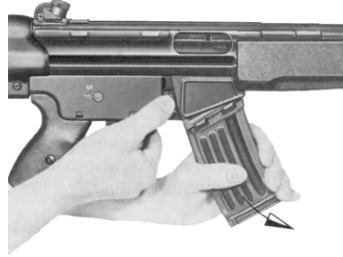
Fig. 31 Removing the magazine
