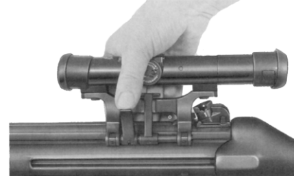
Fig. 54 Attaching the telescopic sight with mount
