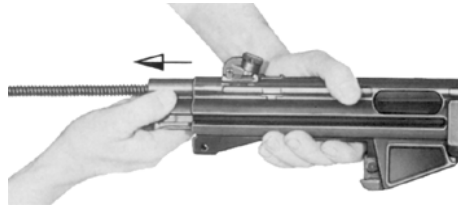
Fig. 37 Removing the bolt assembly
