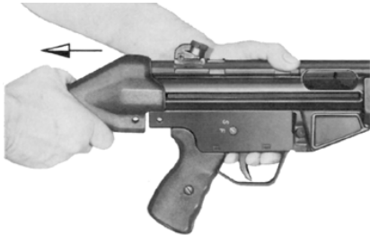
Fig. 36 Removing the buttstock
