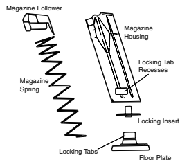
Figure 35C 10 round Civilian Magazine
