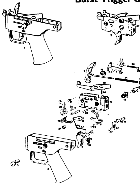
Burst Trigger Group
