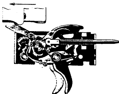
Ill.# 50A - Fully automatic fire
