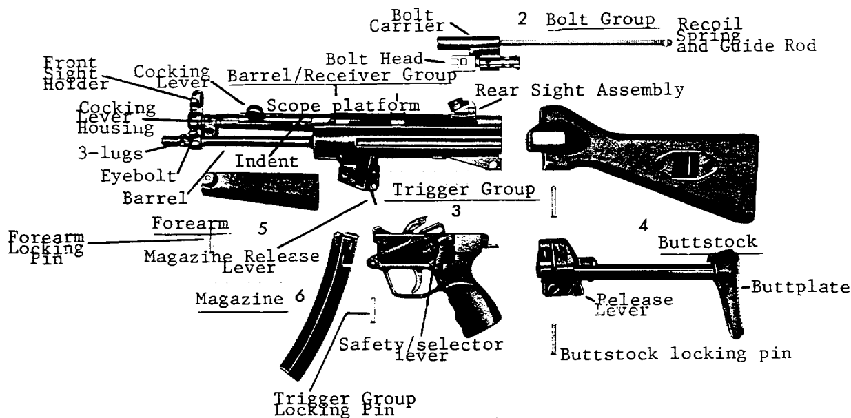
Ill.# 15A - Assembly Groups (MP5A2/A3 pictured)
