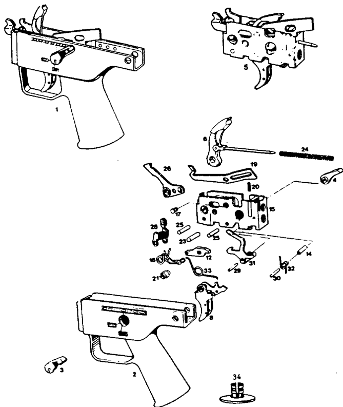
Ambidextrous Trigger Group
