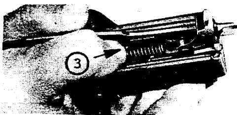
Ill.# 33B - Depressing disassembly lever
