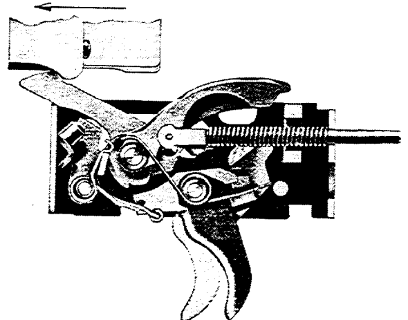
Ill.# 49A - Semiautomatic fire
