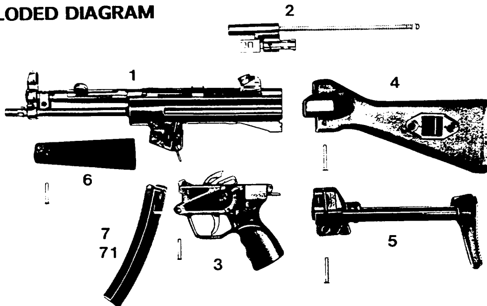
Exploded Diagram # 1 - Assembly Groups
