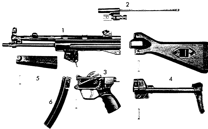
Ill.# 31A - Assembly Groups - MP5A2/A3 pictured
