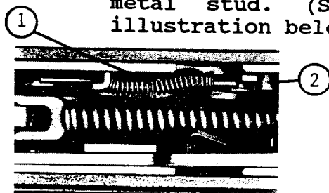
Ill.# 33A - Correct position of burst counting wheel
