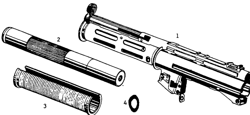
Exploded Diagram # 7
