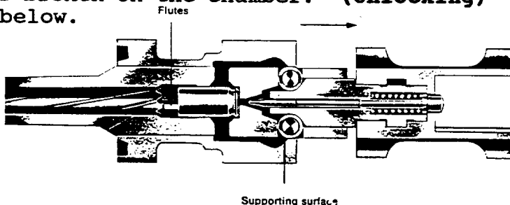
Ill.# 47B - Bolt group in unlocked position
