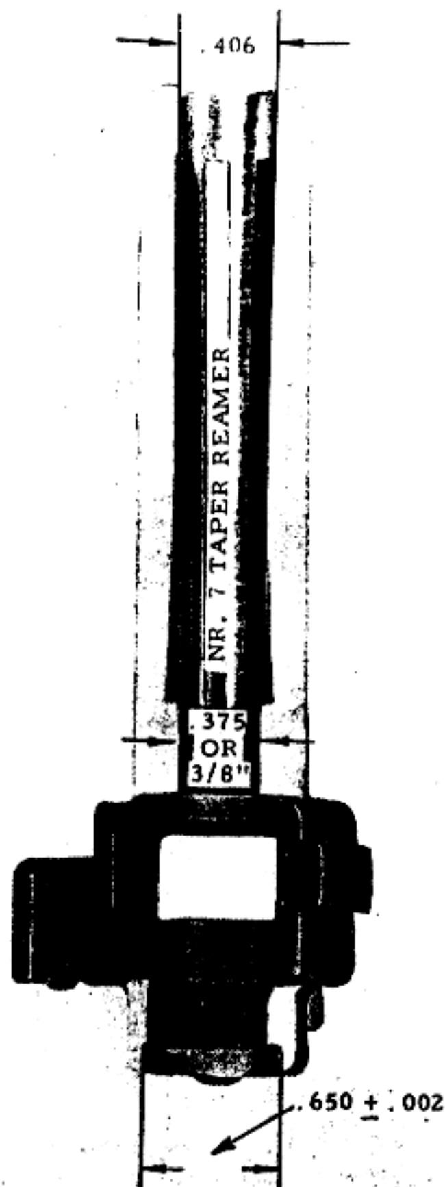
ILLUSTRATION "E 1 " SUPPRESSOR MODIFICATION
