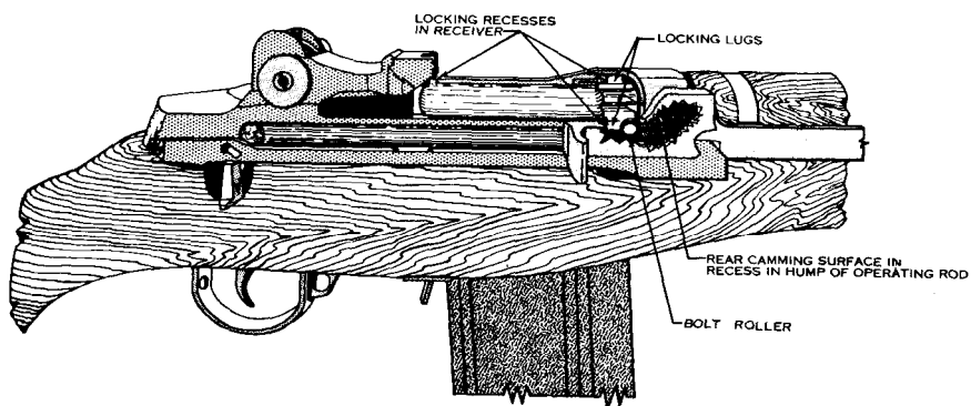
Figure 32. Locking.
