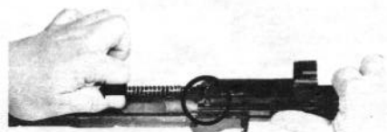
Figure 12. Removing the operating rod spring and operating rod spring guide.
