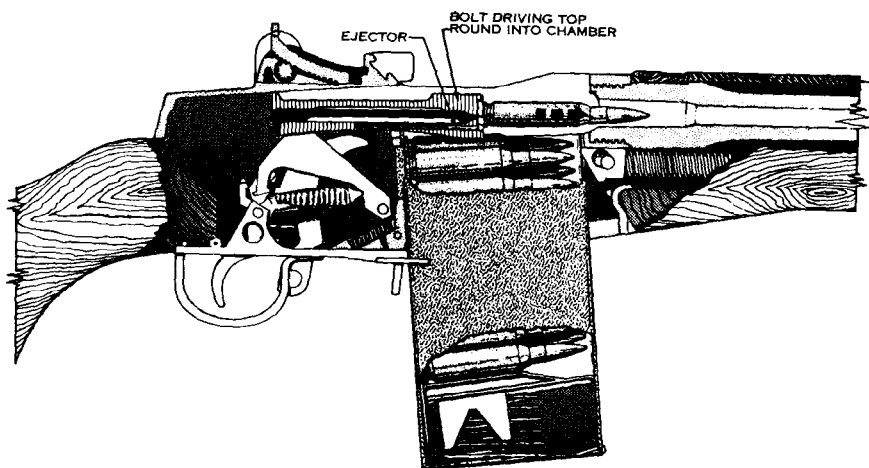
Figure 31. Chambering.
