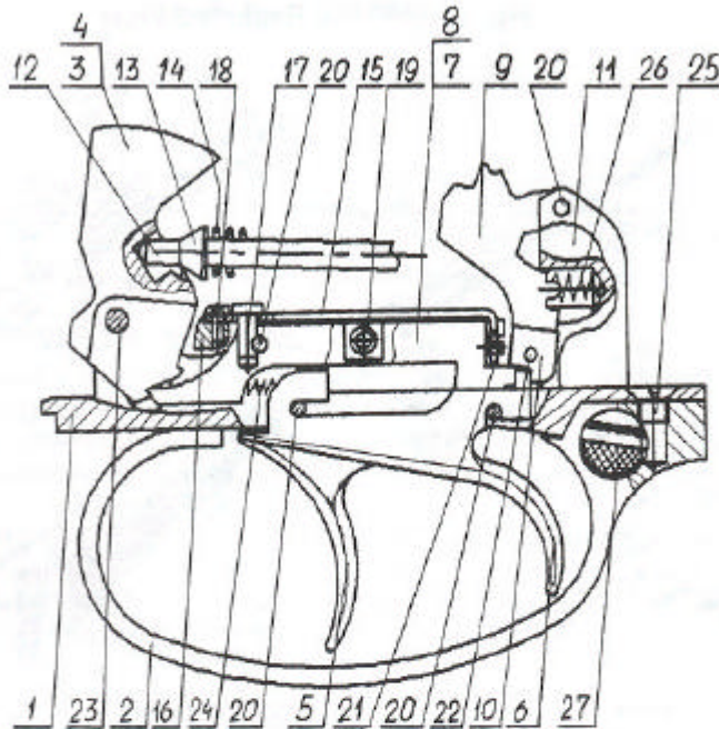
Fig. 2 - Trigger Mechanism
