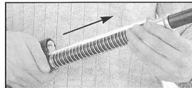
Fig. 17: With the cocking handle removed from the bolt you can grasp the piston, slide the bolt and action bar forward and remove the assembly from the
